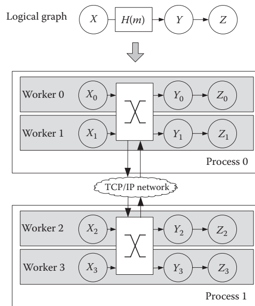
FIGURE 11.19 System architecture of a Naiad cluster.
