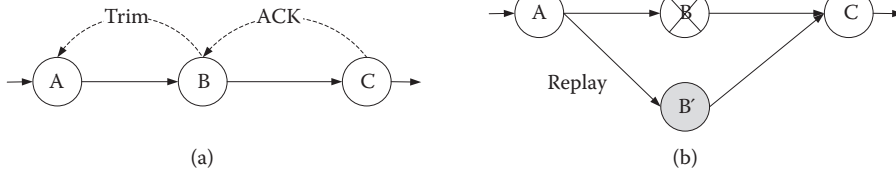
FIGURE 11.7 Upstream backup.
