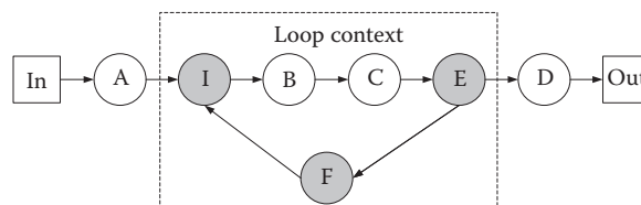
FIGURE 11.18 Timely dataflow graph.
