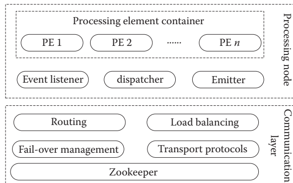
FIGURE 11.12 Processing node.
