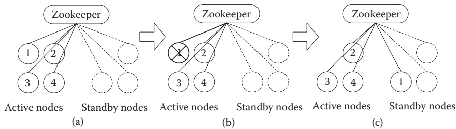
FIGURE 11.13 Fail-over mechanism.
