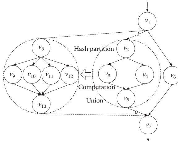
FIGURE 11.17 Resilient substitution.
