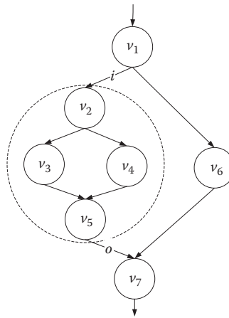
FIGURE 11.16 Streaming DAG and sun-DAG.
